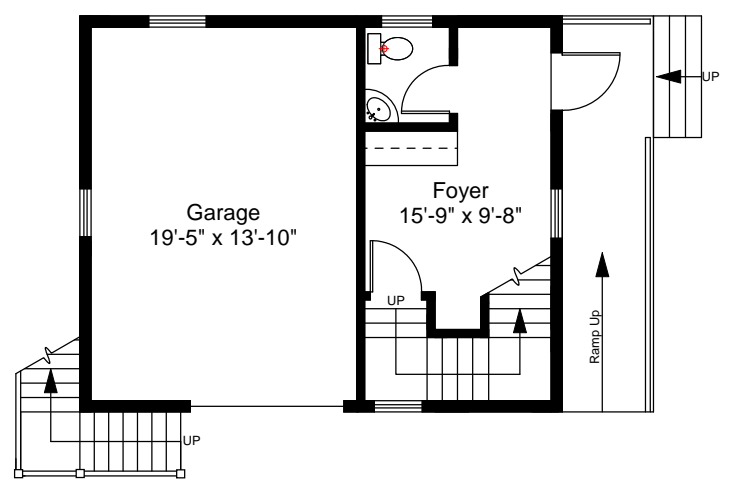
Carriage House - First Floor Plan Ceiling Height = 8'-4"
