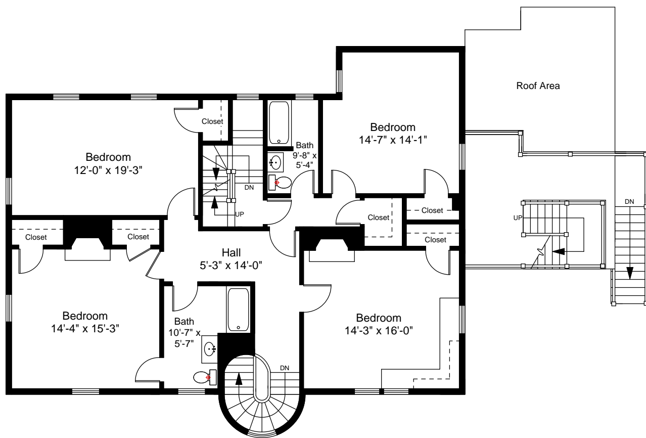
Second Floor Plan Ceiling Height = 8'-3"
