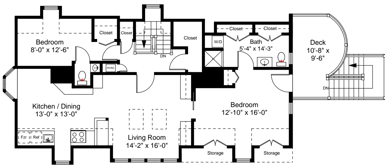
Third Floor Plan Ceiling Height = 8'-2"
