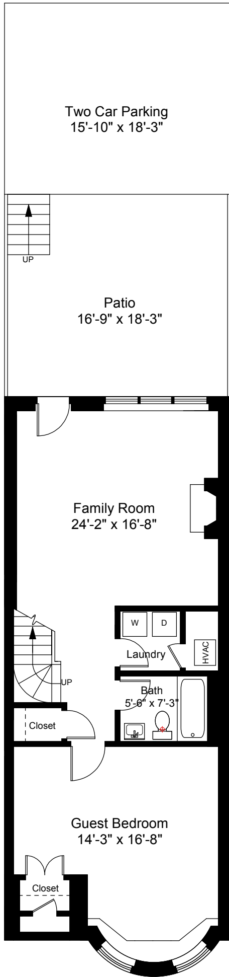
Garden Level Floor Plan Ceiling Height = 8'-5"
