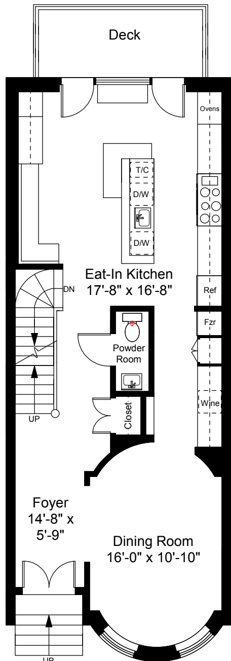
First Floor Plan Ceiling Height = 9'-9"
