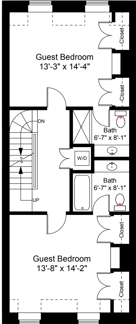
Fourth Floor Plan Ceiling Height =9'-0"
