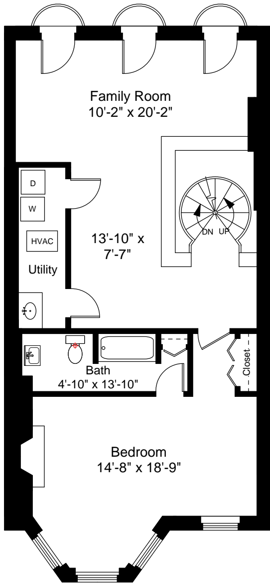
Second Floor Plan Ceiling Height = 9'-2"
