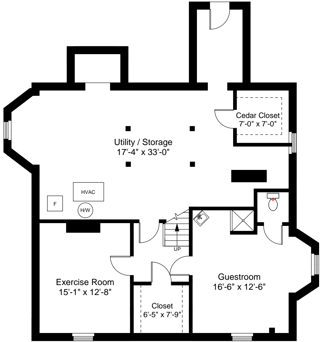
Lower Level Floor Plan Ceiling Height = 6'-11"
