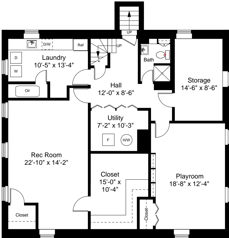
Lower Level Floor Plan Ceiling Height = 7'-2"
