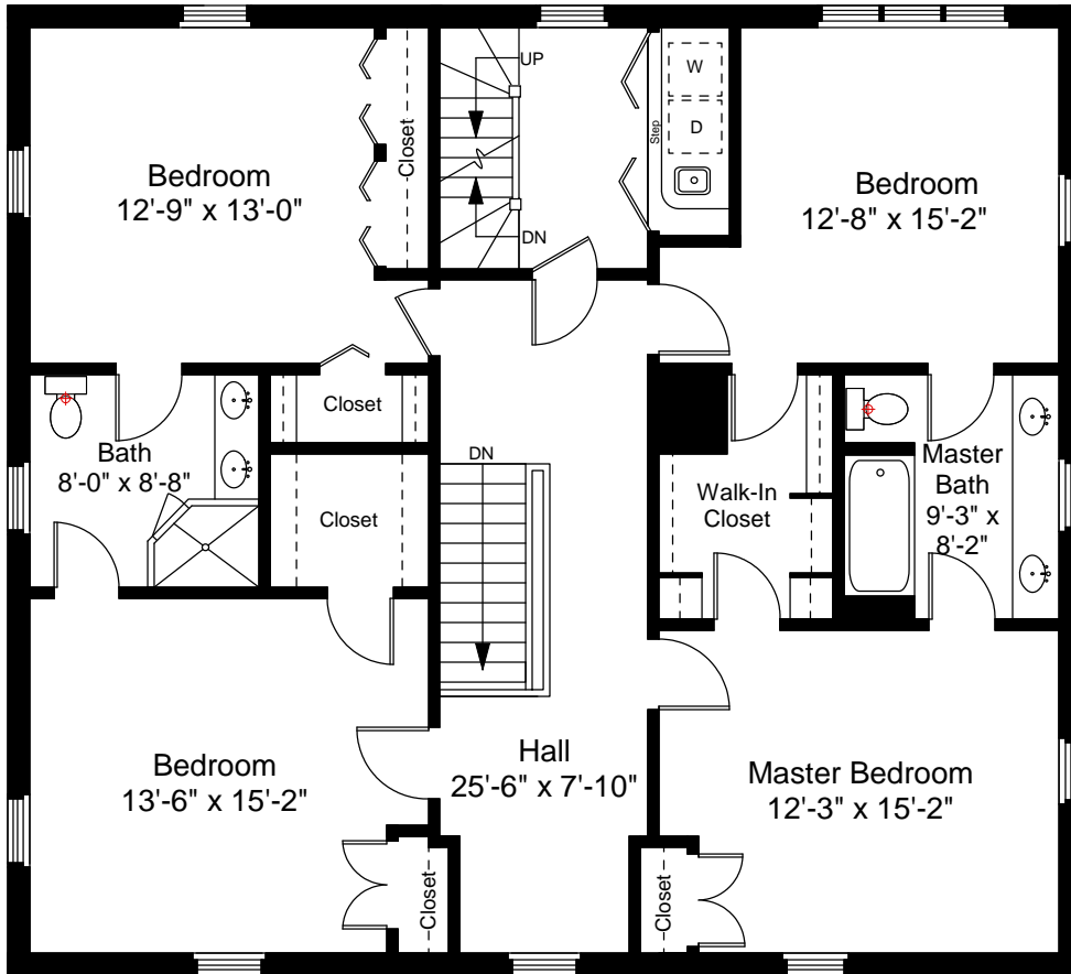
Second Floor Plan Ceiling Height = 7'-1"
