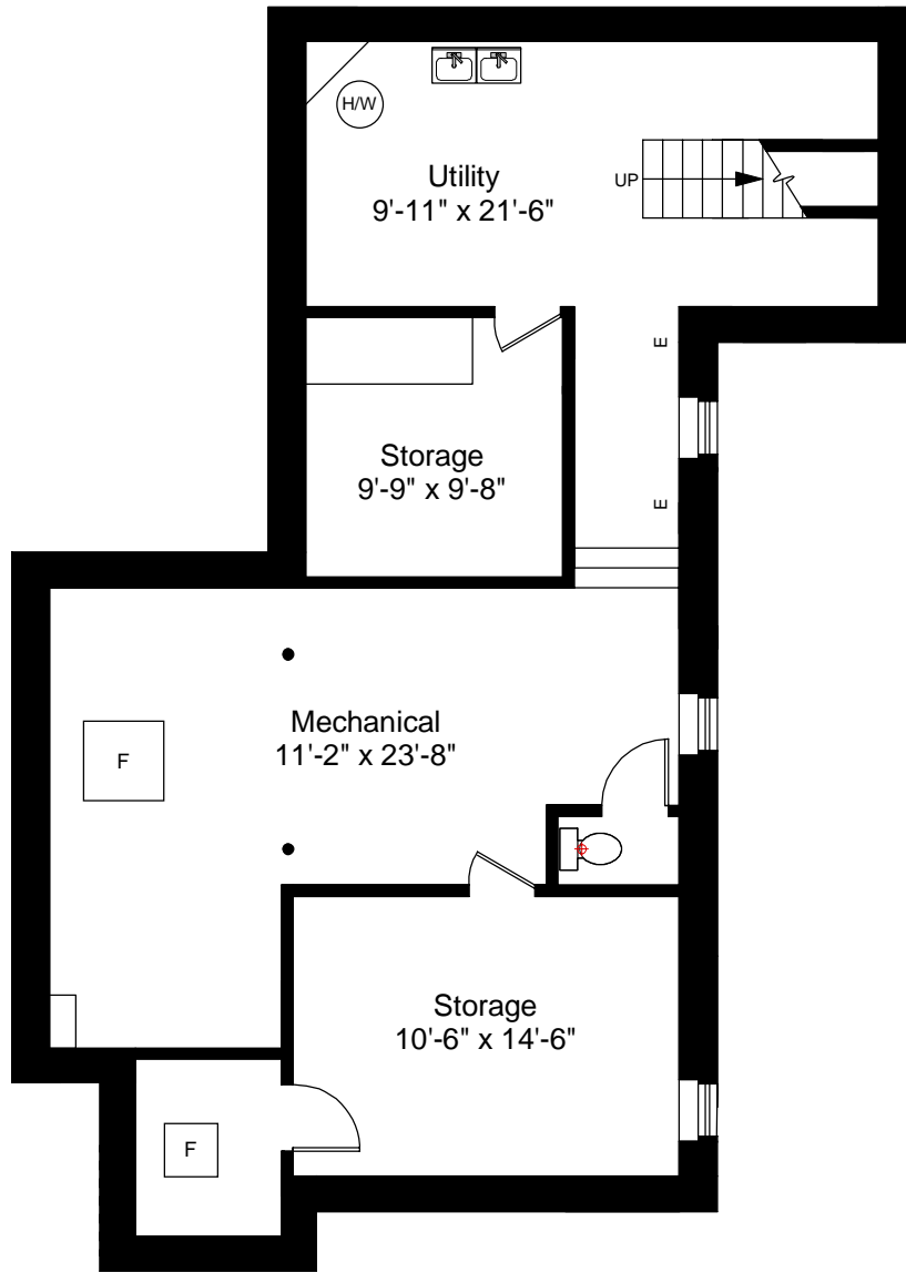
Lower Level Floor Plan Ceiling Height = 7'-6"
