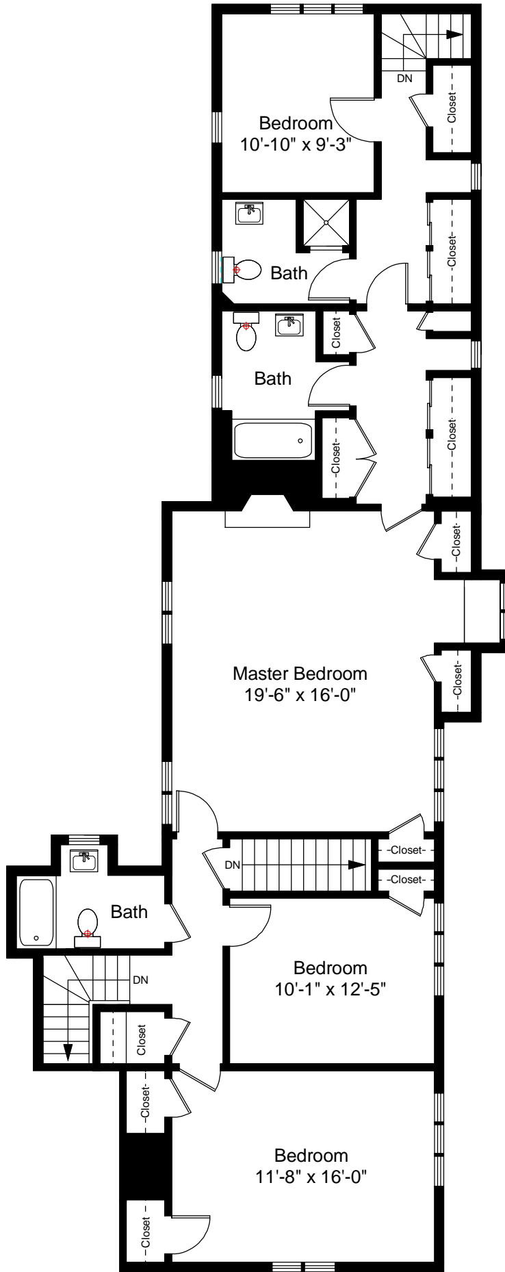
Second Floor Plan Ceiling Height = 7'-7"
