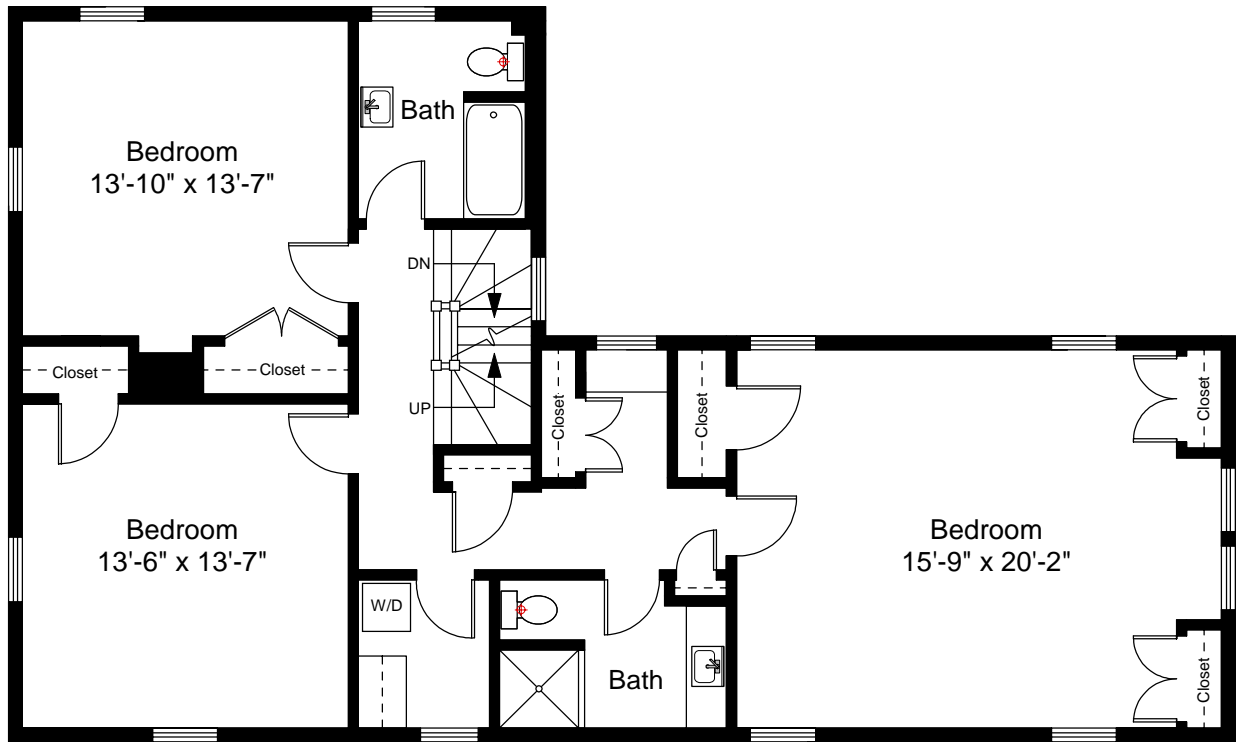
Second Floor Plan Ceiling Height = 8'-3"
