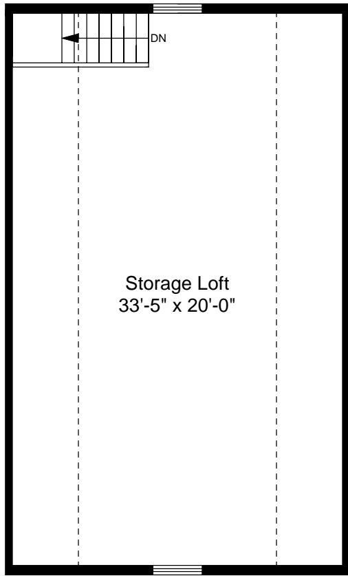
Garage Second Floor Plan Vaulted Ceiling Height = 10'-4"
