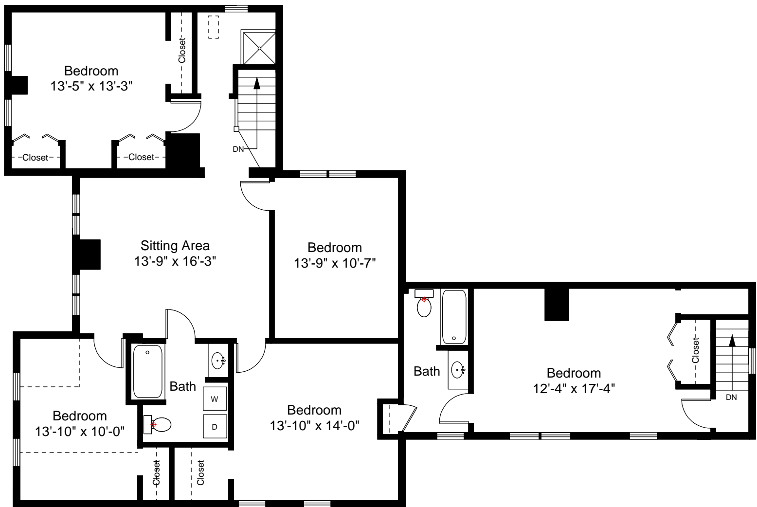
Second Floor Plan Ceiling Height = 7'-3"
