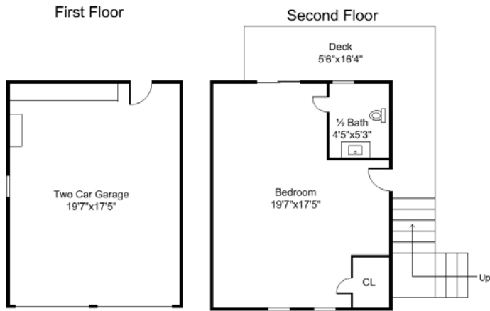
Garage Floor Plan Ceiling Height = 7'-8"
