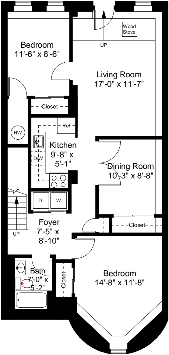
Unit 1 Floor Plan Ceiling Height = 8'-6"
