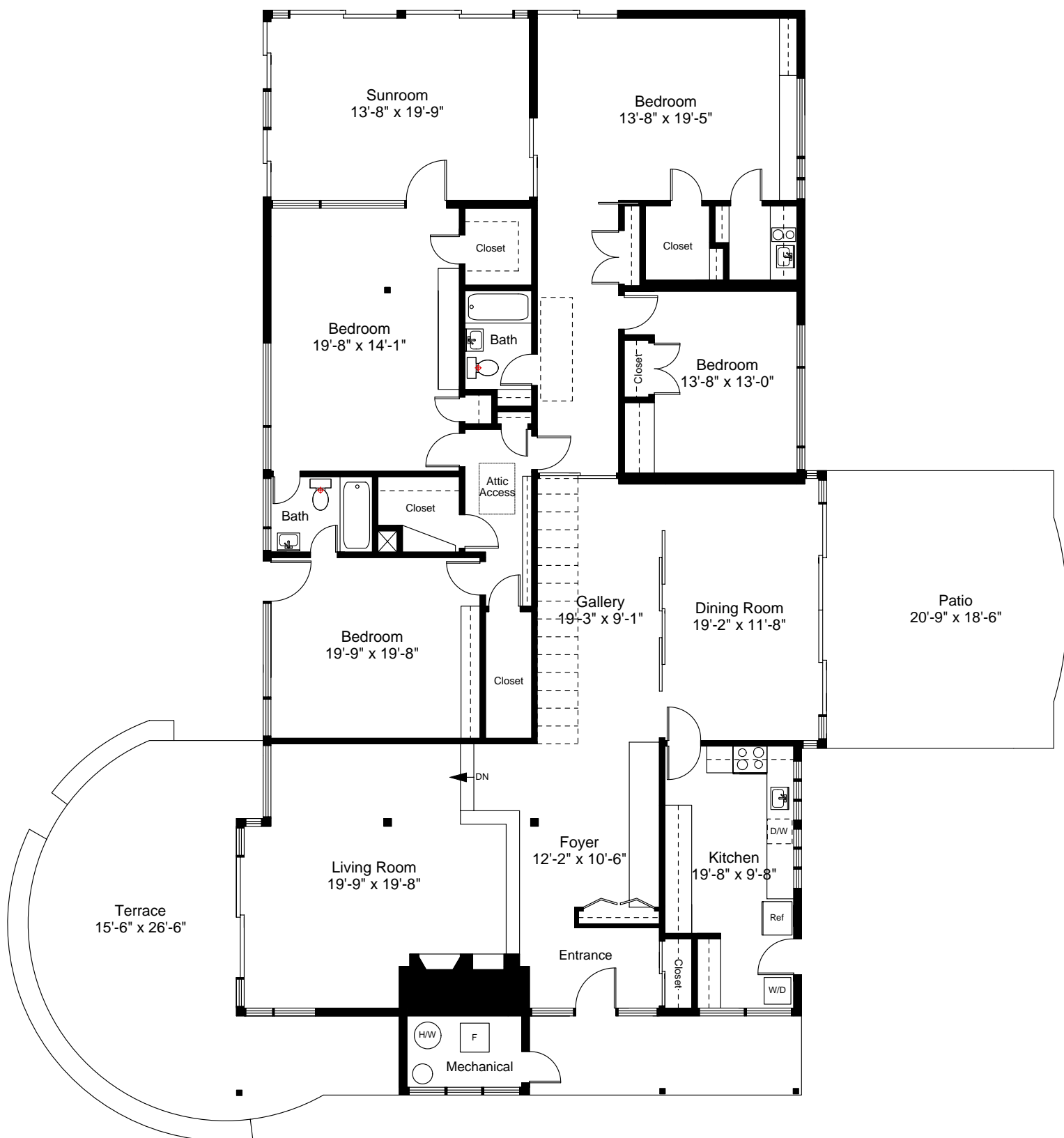
Floor Plan Vaulted Ceiling Height = 11'-6"
