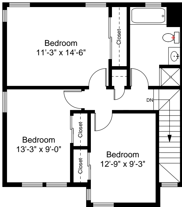
Second Floor Plan Ceiling Height = 8'-8"
