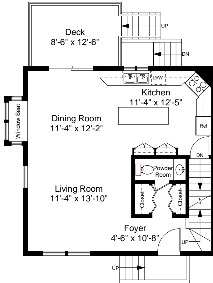
First Floor Plan Ceiling Height = 8'-8"
