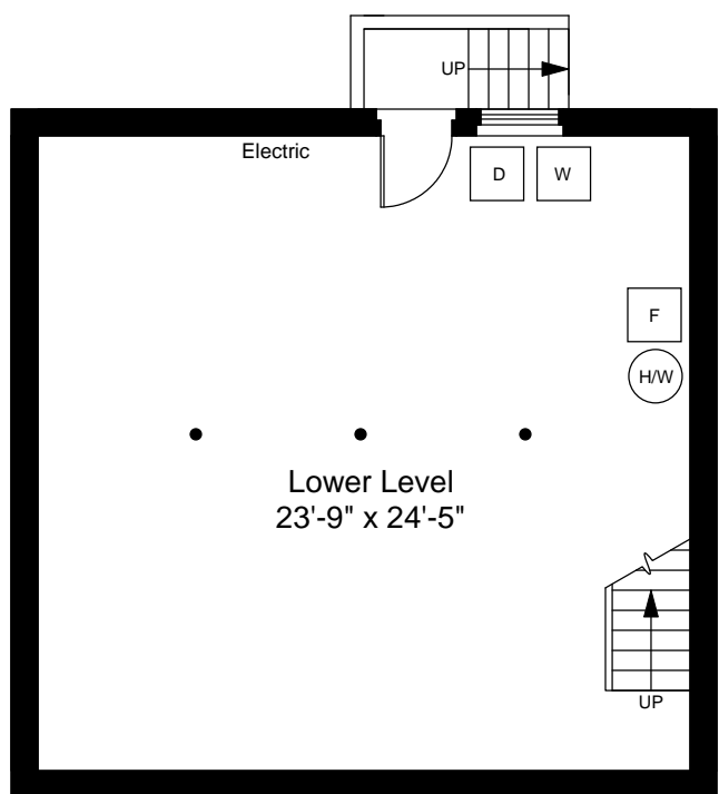
Lower Level Floor Plan Ceiling Height = 7'-5"
