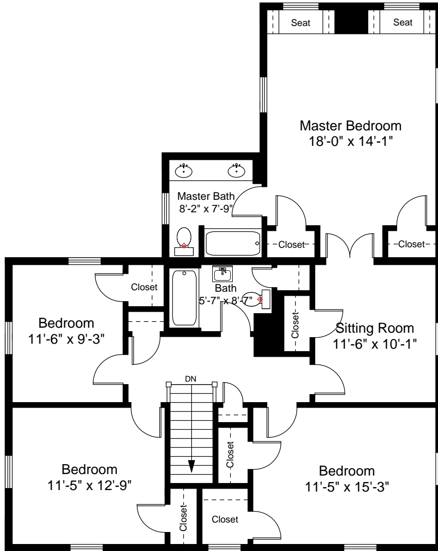
Second Floor Plan Ceiling Height = 8'-0"
