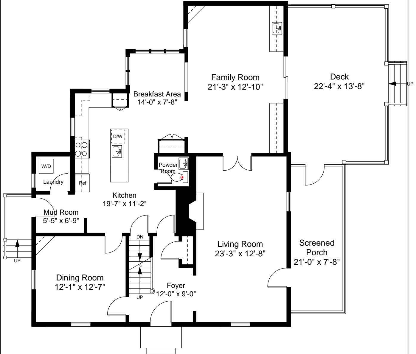
First Floor Plan Ceiling Height = 8'-0"
