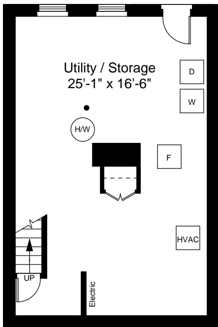
Basement Floor Plan Ceiling Height = 6'-6"
