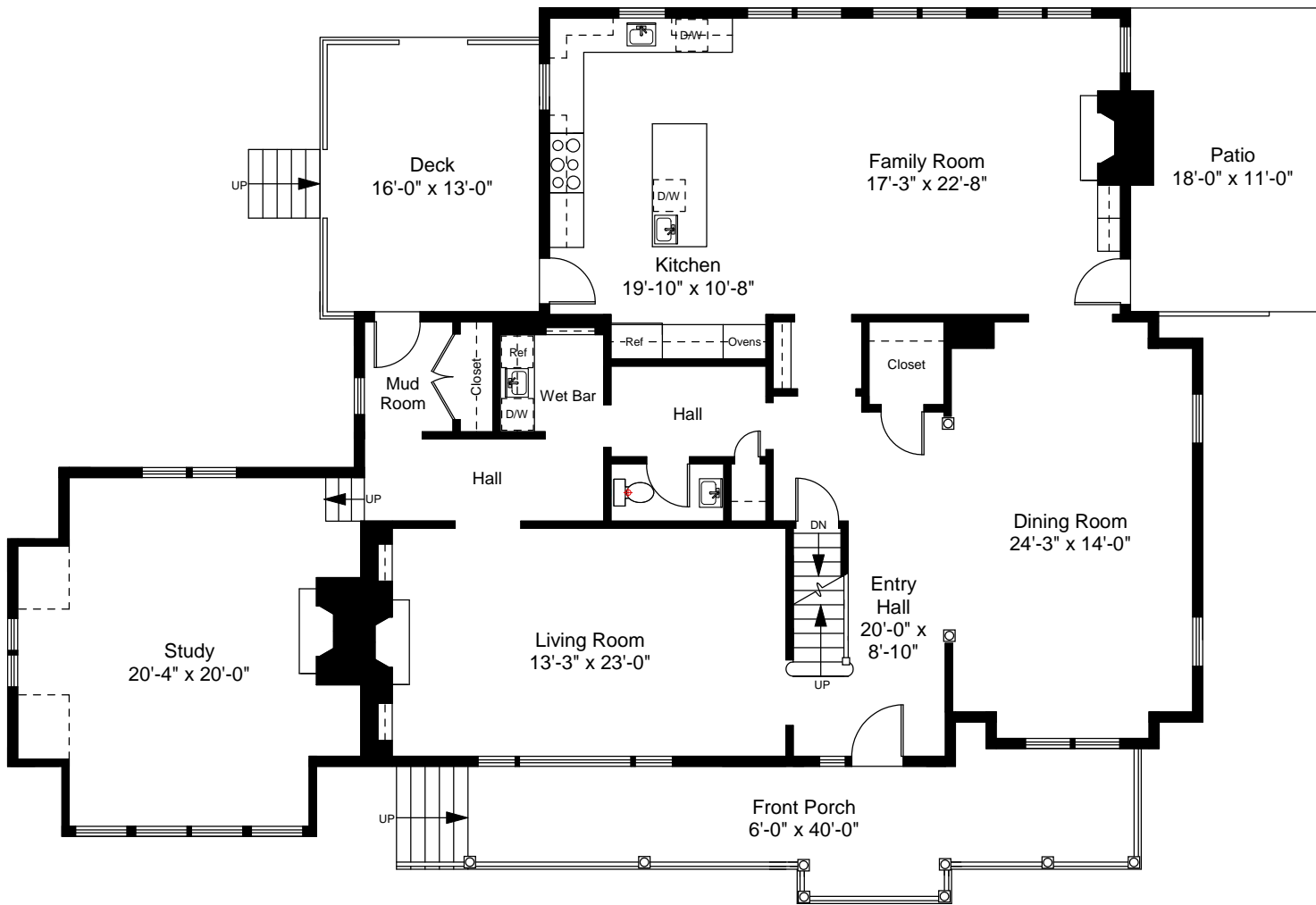
First Floor Plan Ceiling Height = 7'-6"
