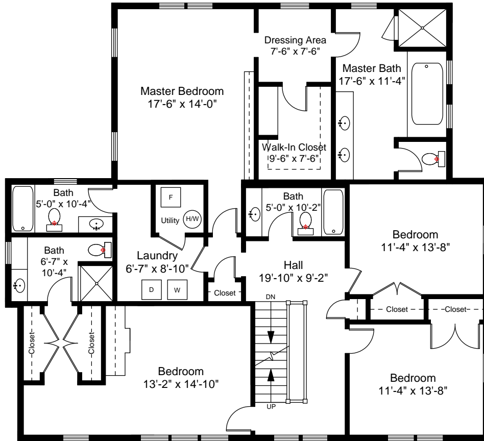
Second Floor Plan Ceiling Height = 7'-9"
