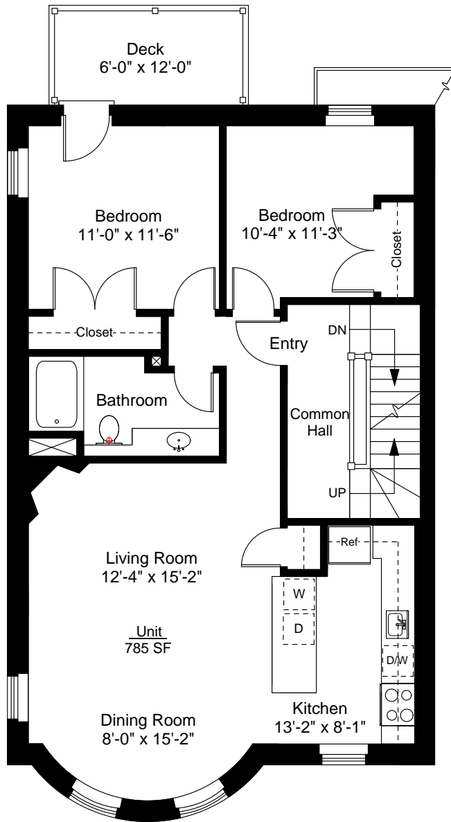
Unit Floor Plan Ceiling Height = 10'-2"
