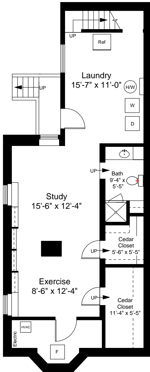
Lower Level Floor Plan Ceiling Height = 8'-1"
