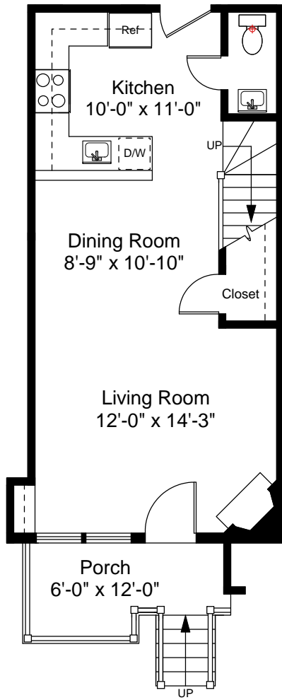
First Floor Plan Ceiling Height = 7'-6"
