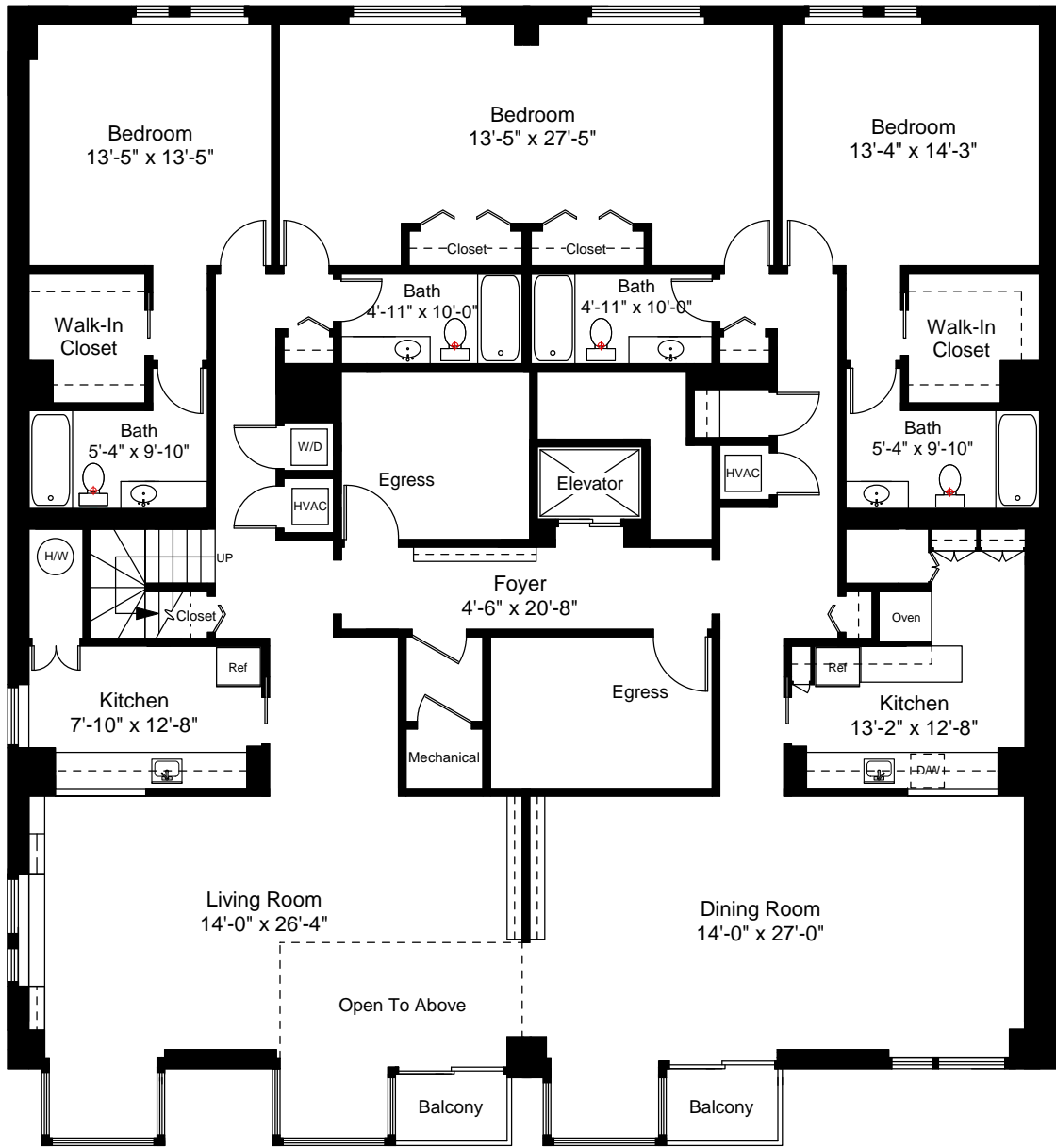
First Floor Plan Ceiling Height = 8'-0"
