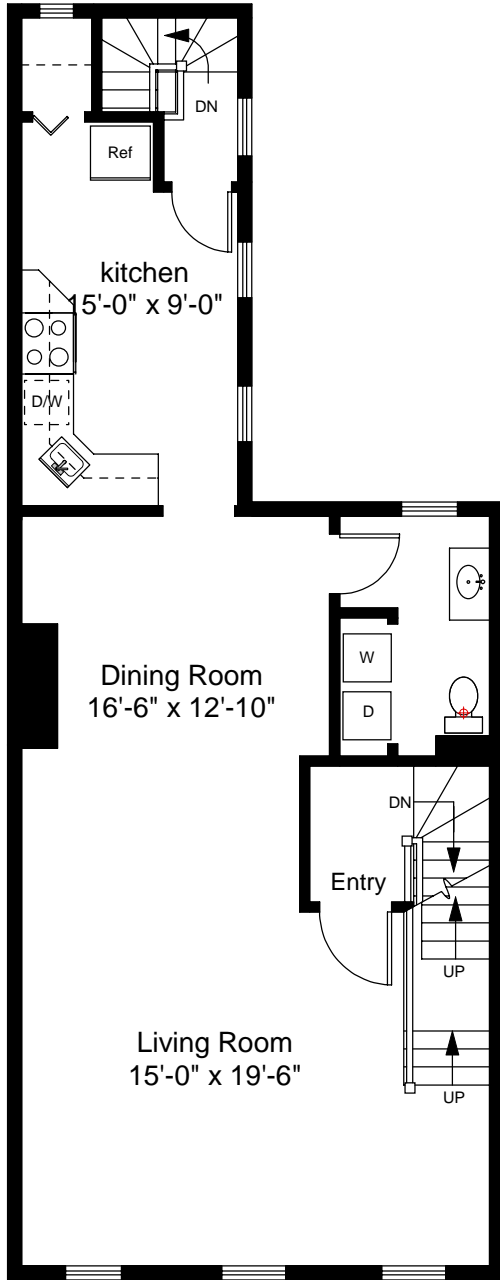
First Floor Plan Ceiling Height = 9'-6"
