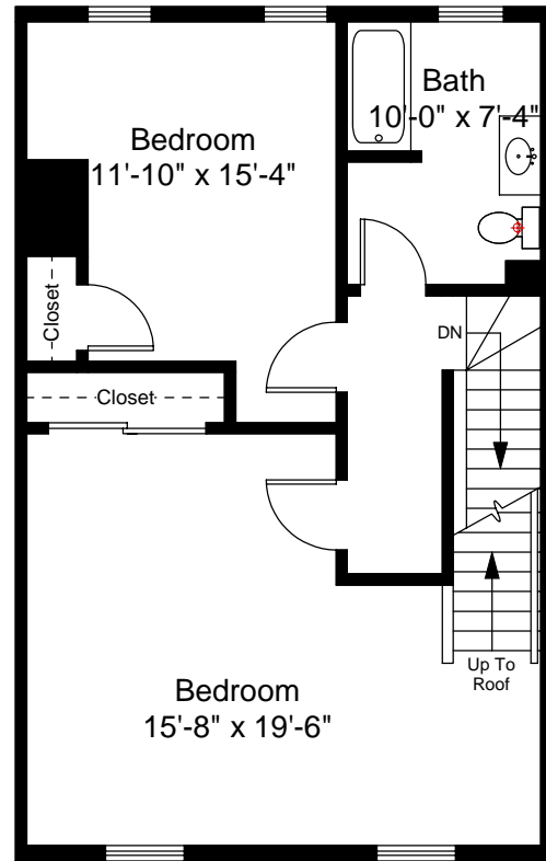
Second Floor Plan Ceiling Height = 9'-8"
